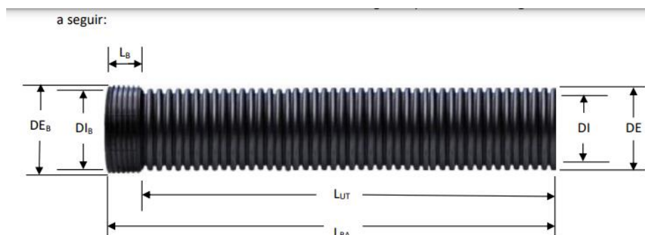
Figura 4 - Tubo KNTS Drain
